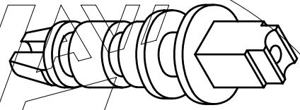
PICK-UP NOZZLE PA 2747/50 PHIL
