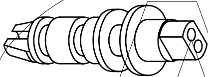
PICK-UP NOZZLE PA 2745/80 PHIL
